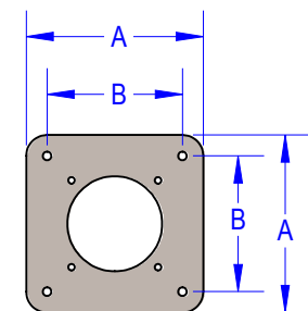
MOUNTING DETAIL
