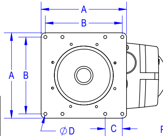
SECTION A-A: MOUNT DETAIL
