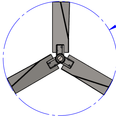
SECTION B-B: IMPELLER DETAIL
