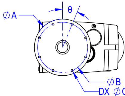
SECTION A-A: MOUNT DETAIL
